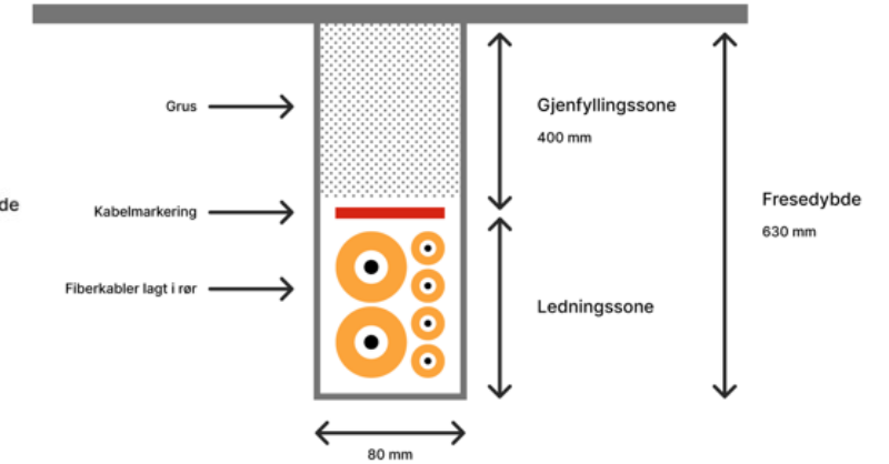
Kabelgrøft - Maskingraving
