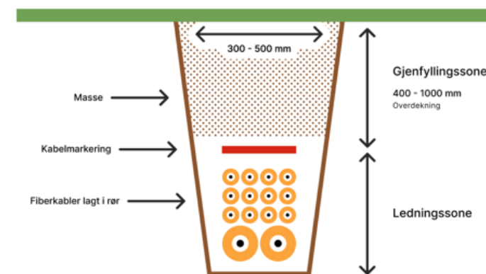
Kabelgrøft - Maskingraving
