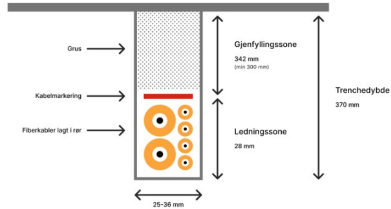
Kabelgrøft - Maskingraving
